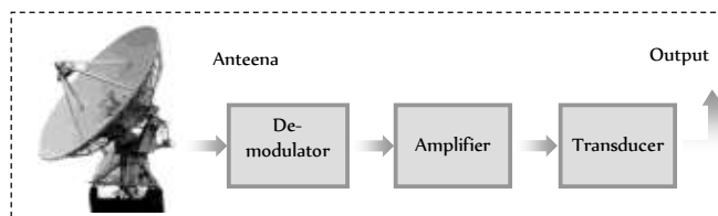
Fig. 28.3 : Receiver
