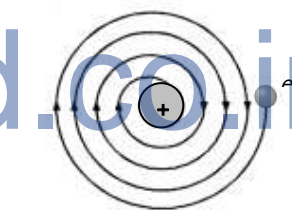
Instability of atom
